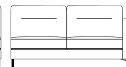
189PL/R W189 x H90 x D93 cm
