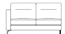
149PL/R W149 x H90 x D93 cm
